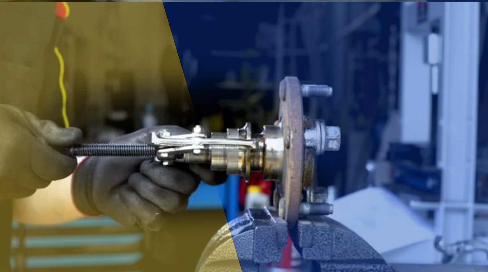
Gear Puller, 2 Jaws Drop Forged Cr-V Steel Jaws
